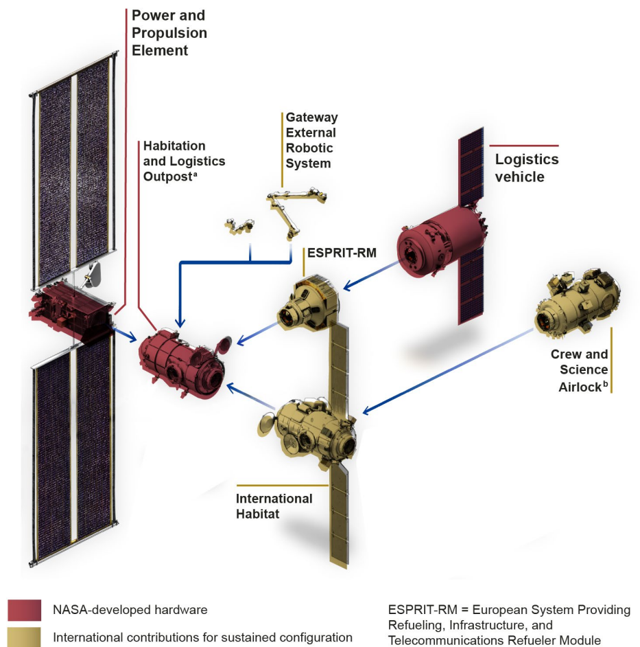
Figure 1: Illustration of the Gateway Sustained Configuration
