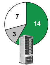
Underutilized servers
