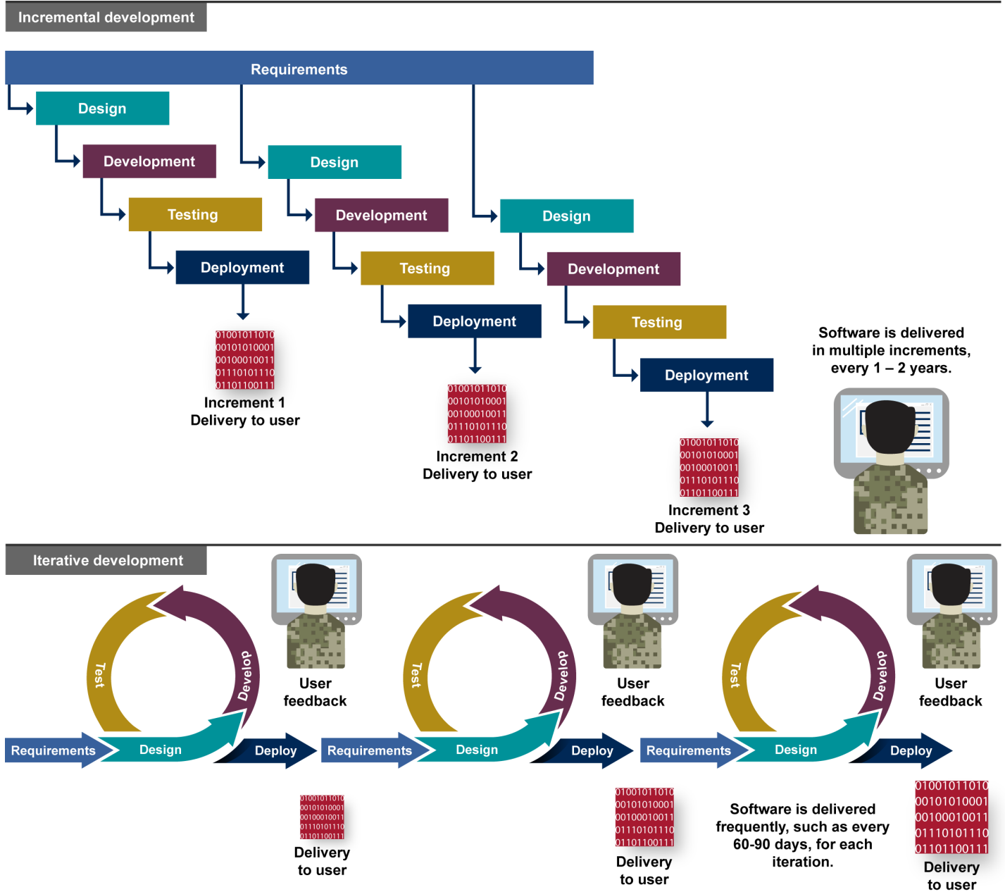
Figure 3: Comparison of Incremental and Iterative Software Development
