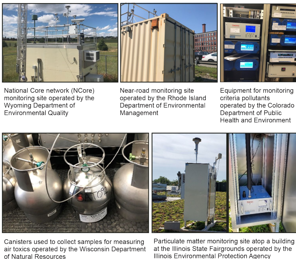
Figure 6: Examples of Air Monitoring Sites and Monitoring Equipment
