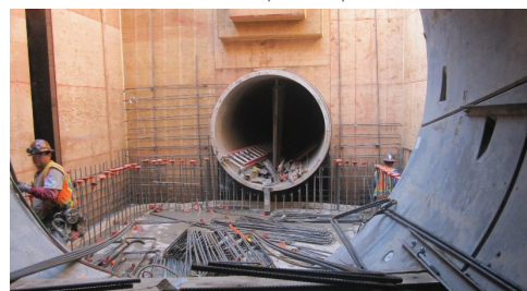
Construction of New Sunnydale Tunnel in 2011
