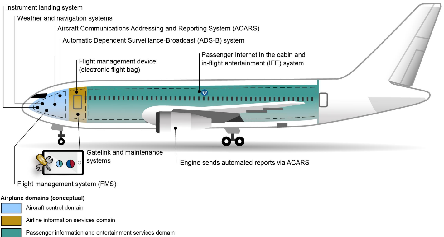
Figure 1: Key Systems Connections to Commercial Airplanes
