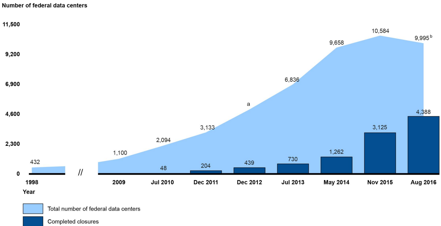
Figure 2: Total Number of Reported Federal Data Centers and Closures through August 2016
