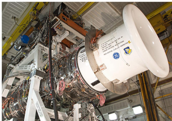
Figure 17: Close Collaboration Led to Successful Development of the Air Force's Adaptive Engine Technologies
