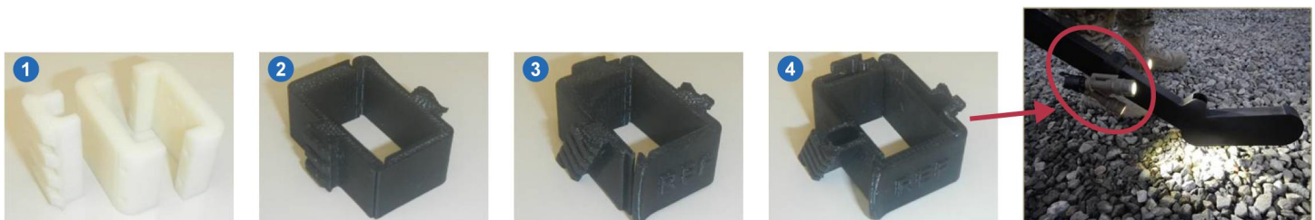
Figure 6: Army Flashlight Mounting Brackets Additively Manufactured
