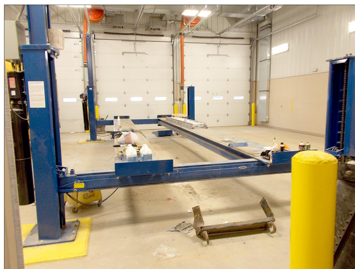
Figure 8: Exterior and Interior of Recently-Constructed Bus Maintenance Building Where Door Does Not Close When a Large School Bus Is On Hydraulic Lift
